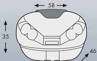
Top case Journey 52 Capacity: 52 litres Weight: 4,8 kg
